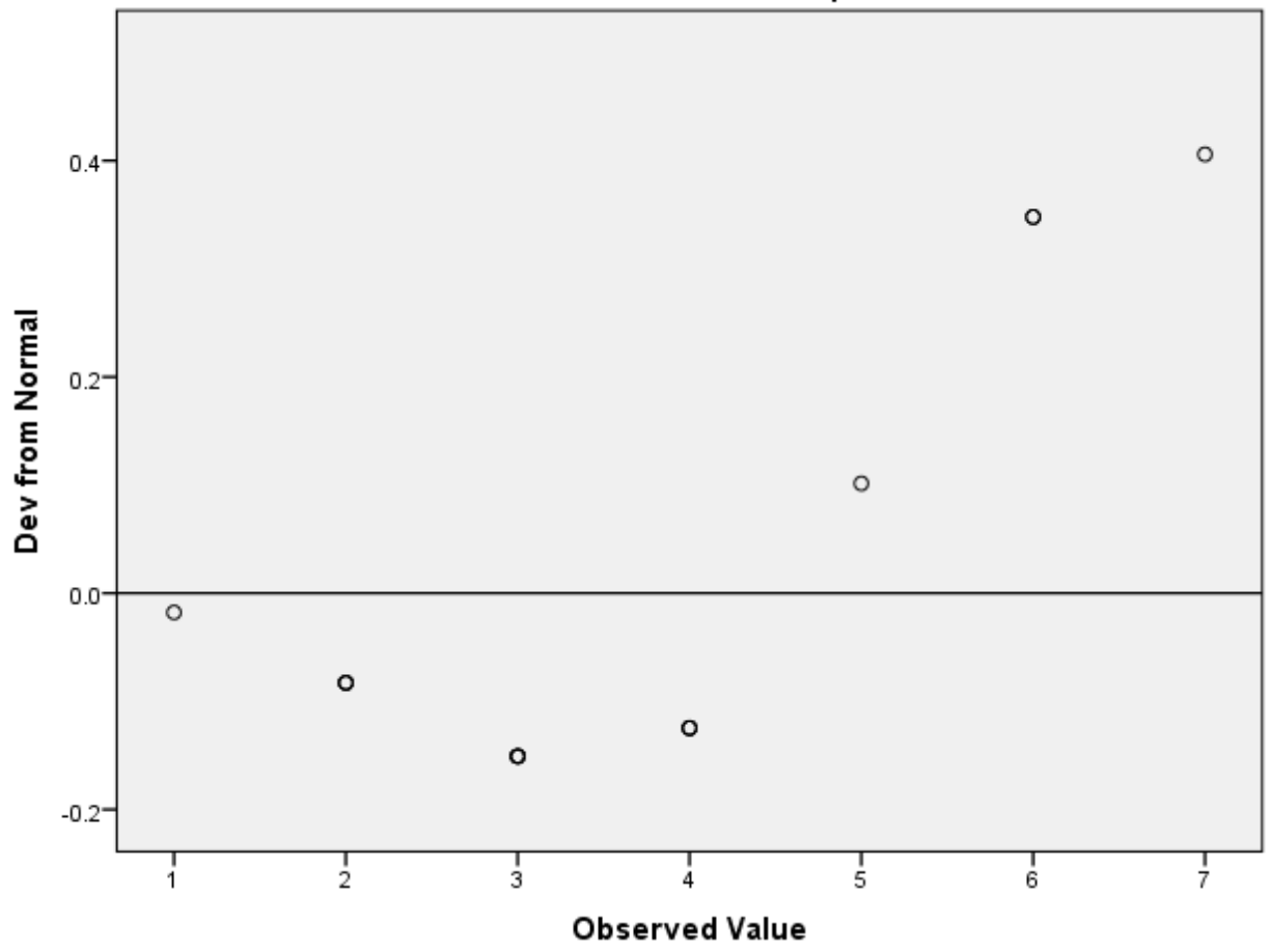
Detrended Normal Q-Q Plot of post
