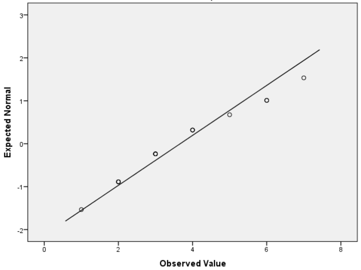
Normal Q-Q Plot of post
