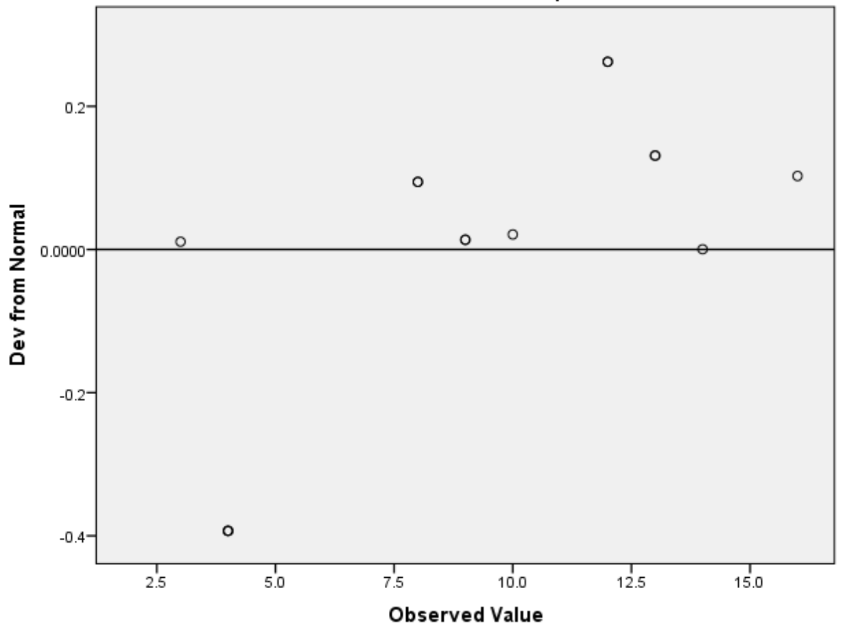
Detrended Normal Q-Q Plot of pre
