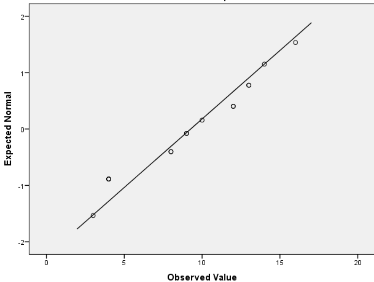
Normal Q-Q Plot of pre
